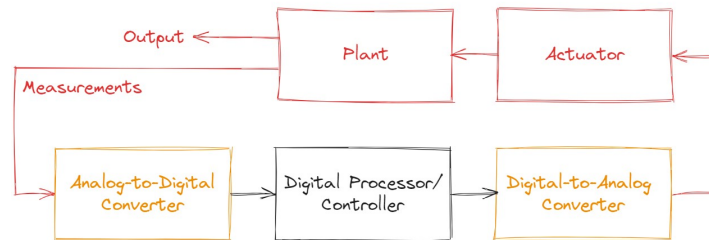
FIGURE 4.1: A block diagram of a digital system.
