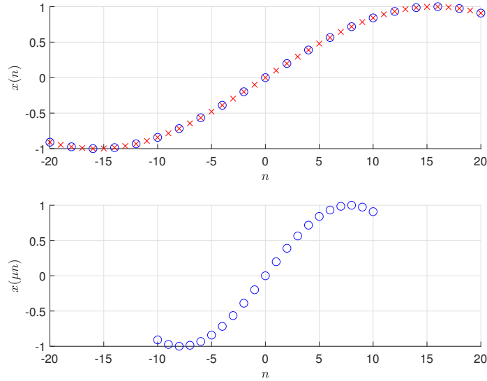
FIGURE 4.4: A demonstration of down-sampling.
