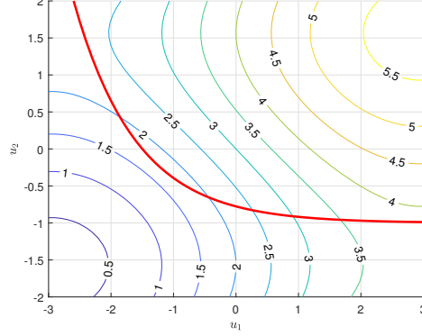
FIGURE 6.1: Static optimization with equality constraint demonstration.
